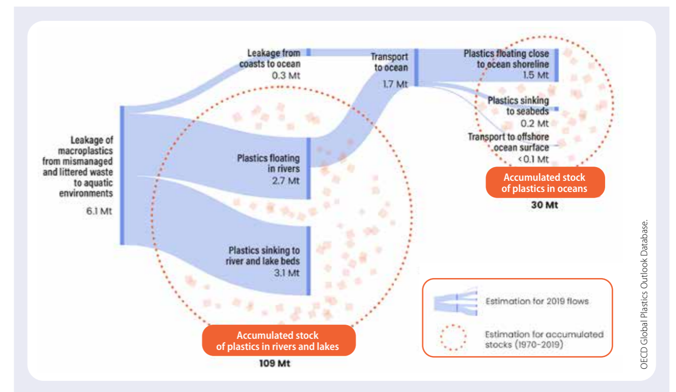
Figure 6. Rivers accumulate leaked plastics and are pathways to the ocean Million tonnes (Mt), 2019
