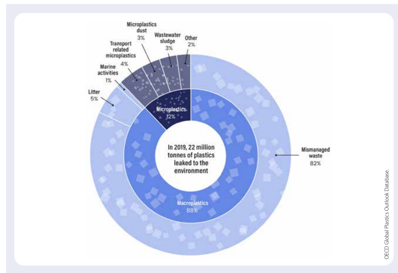
Figure 5. Global leakage of macro-and microplastics to the environment is estimated at 22 million tonnes Million tonnes (Mt), 2019
